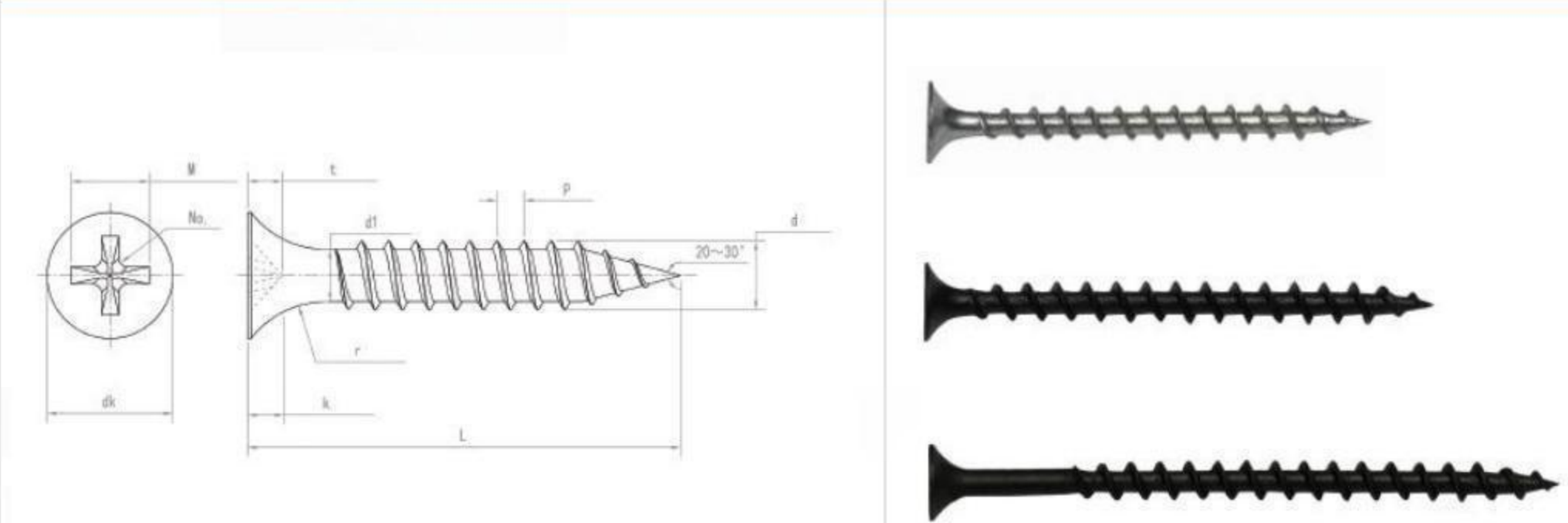
Phillips Bugle Head Drywall Screw Coarse Thread
