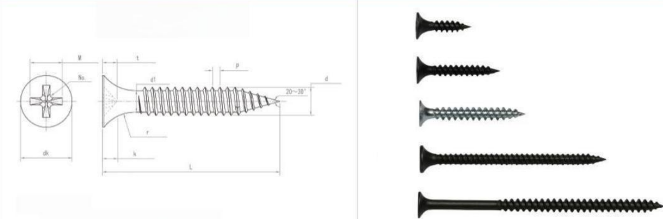
Phillips Bugle Head Drywall Screw Fine Thread
