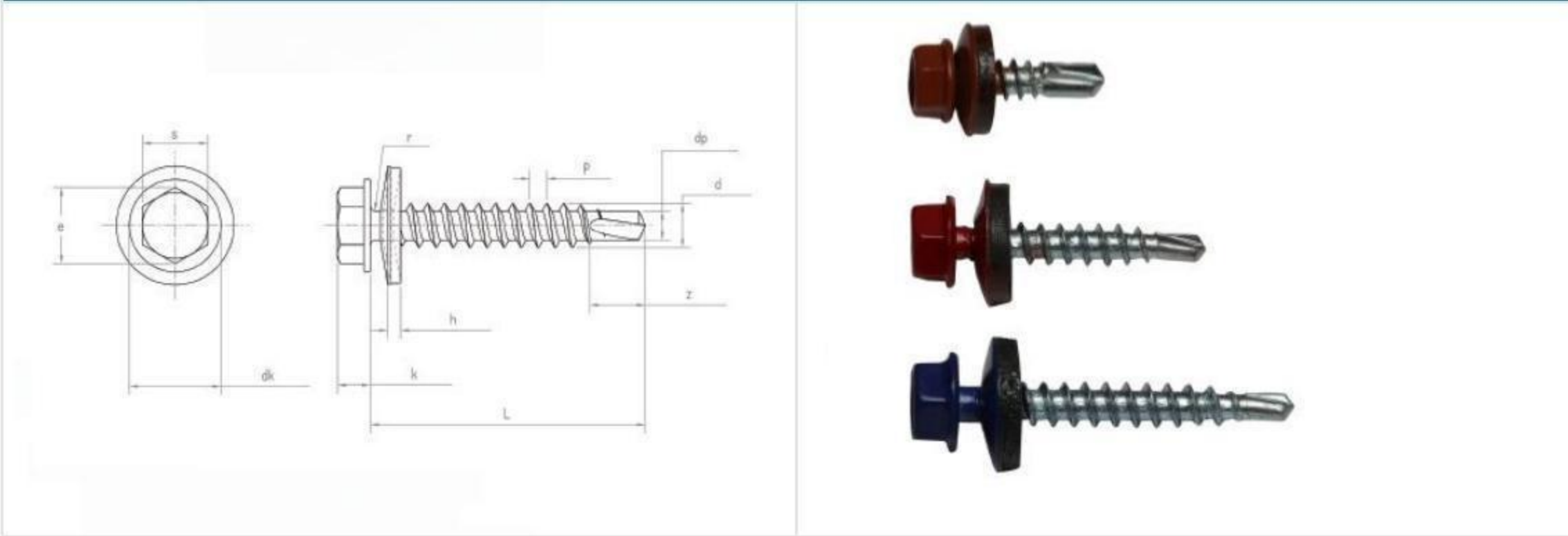
Hex Washer Head Self-Drilling screw with EPDM Washer,Colored head
